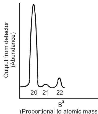
Fig. The mass spectrum of naturally occurring neon, showing three isotopes whose atomic mass number are 20, 21 and 22. The larger the peak, the more abundant the isotope.
