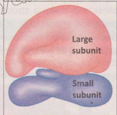
FIGURE 3.8: Ribosome
