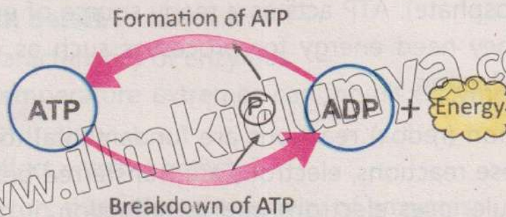
FIGURE 8.2: ATP-ADP Cycle
