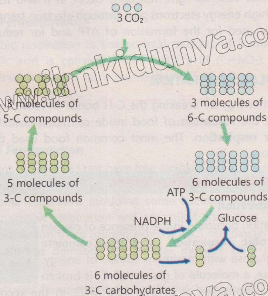
FIGURE 8.4: Dark reactions of photosynthesis
